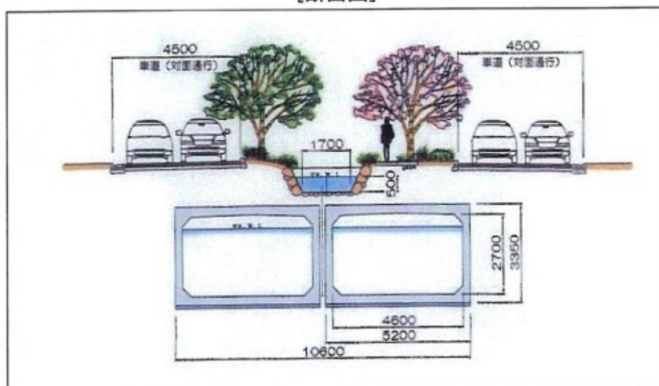
[断面図]
